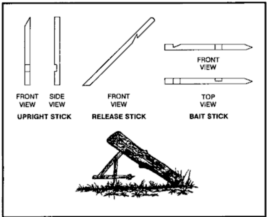
Figure 8-12. Figure 4 deadfall.
