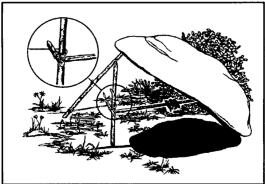
Figure 8-13. Paiute deadfall.
